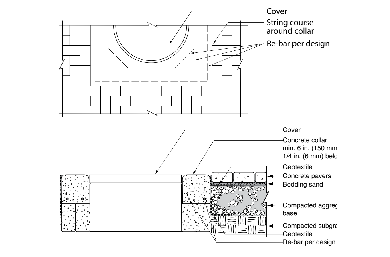
Figure 9. Utility cover.
