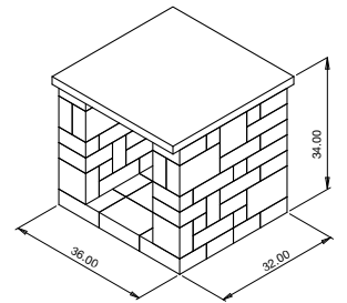
Woodbox/Stand
