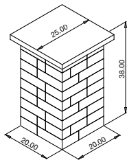
20" Pillar
