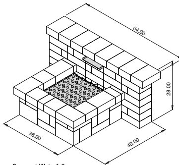
Compact Waterfall
