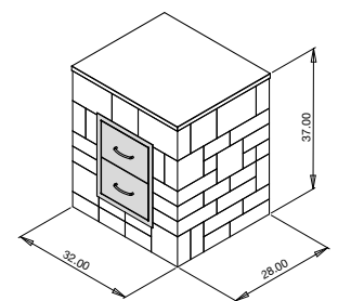
Two Drawer Cabinet
