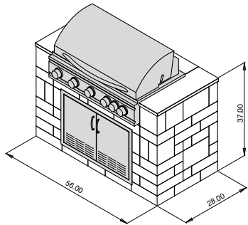
40" Sizzler Grill Cabinet
