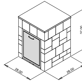
Trash Cabinet
