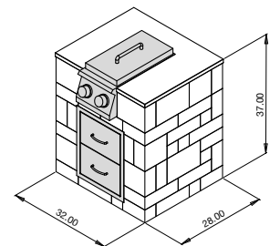
Side Burner Cabinet
