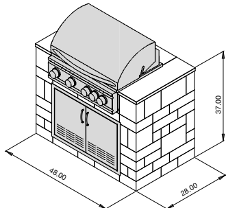
32" Sizzler Grill Cabinet
